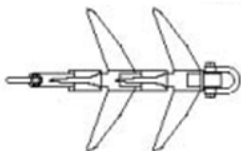
LSP ASSEMBLED SIZE "C"
